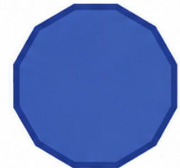
Dodecagon 12 sides
