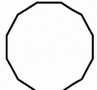
Dodecagon 12 sides
