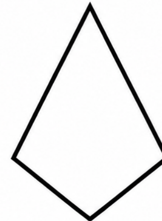
Kite
