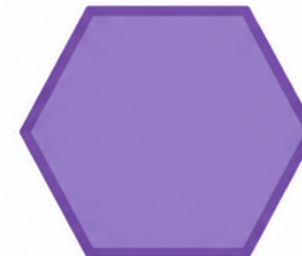
Hexagon 6 sides
