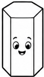
Hexagonal prism
