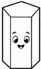
Pentagonal prism
