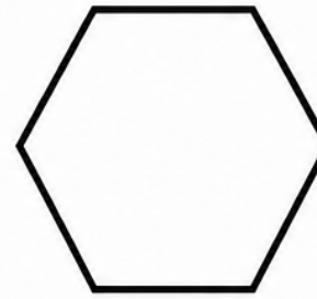
Hexagon 6 sides
