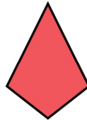
Kite
