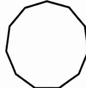
Hendecagon 11 sides
