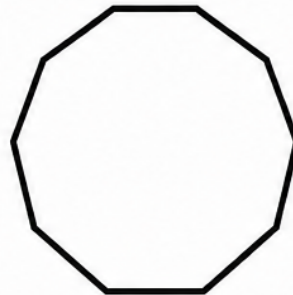
Decagon 10 sides
