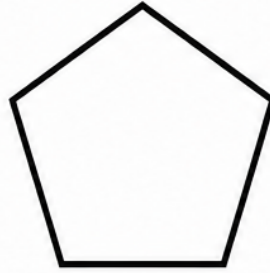
Pentagon 5 sides
