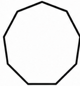
Nonagon 9 sides
