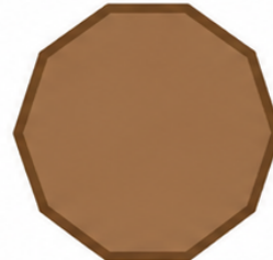
Decagon 10 sides
