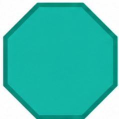
Octagon 8 sides
