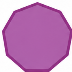
Nonagon 9 sides
