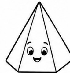
Pentagonal pyramid
