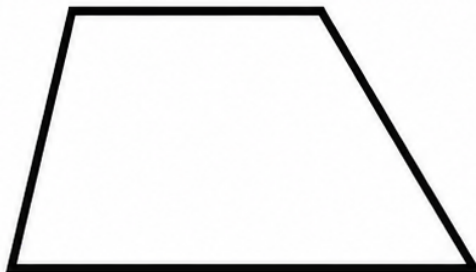
Trapezoid
