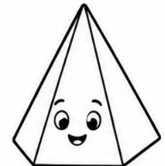
Hexagonal pyramid
