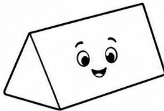
Triangular Prism
