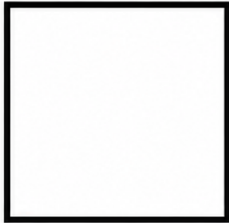
Square
