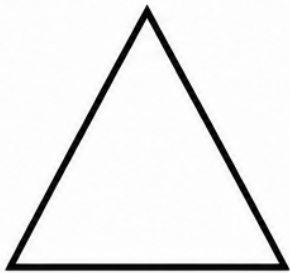
Triangle 3 sides
