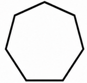
Heptagon 7 sides
