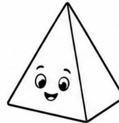
Square pyramid
