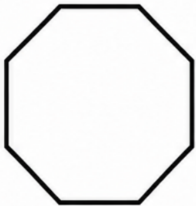
Octagon 8 sides
